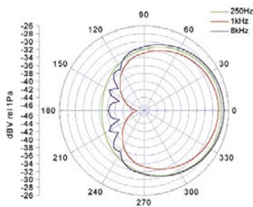
Broadcaster Polar Response
