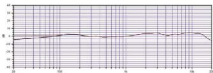
Broadcaster Frequency Response
